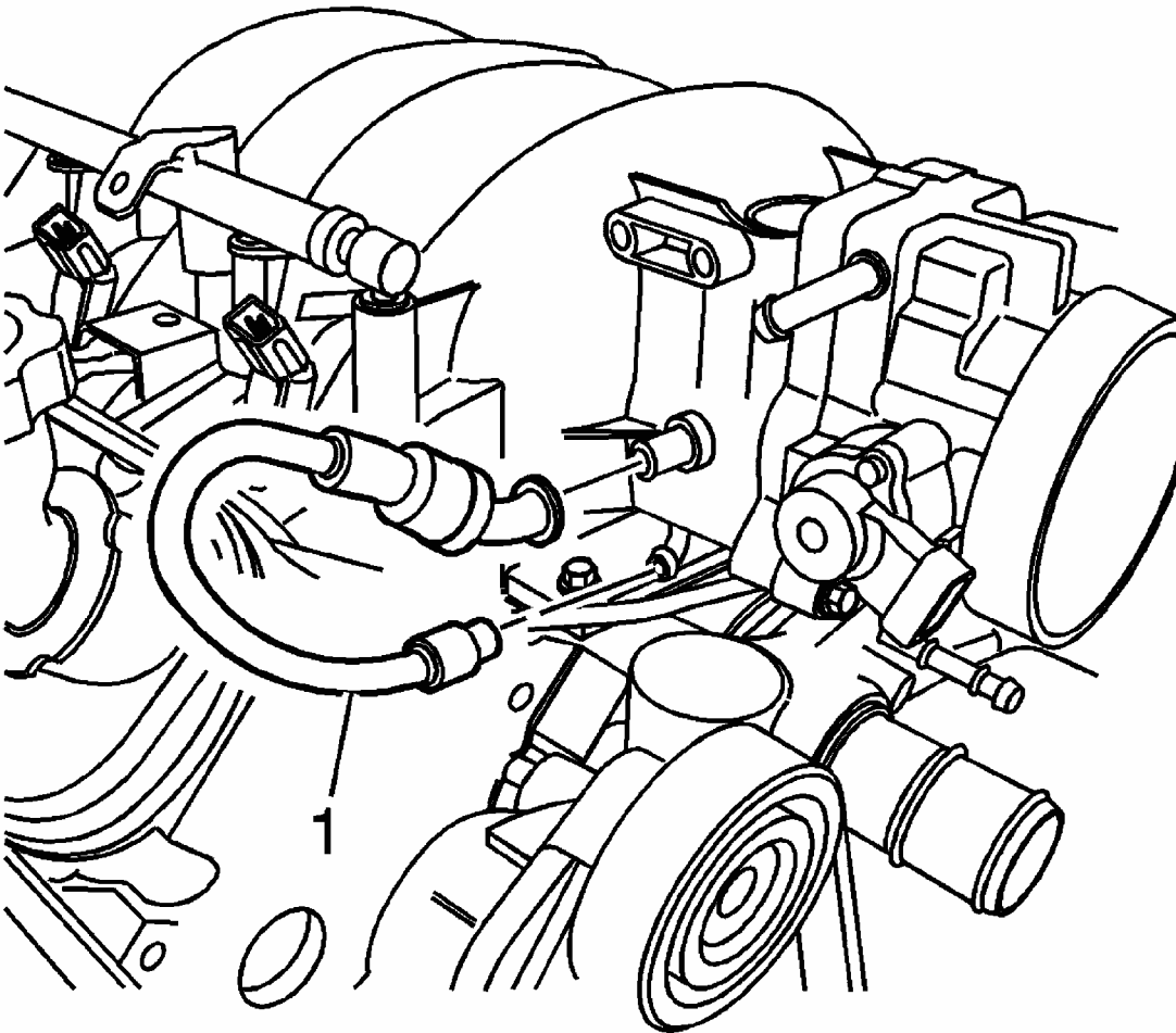
Fig. 50: PCV Valve Hose
