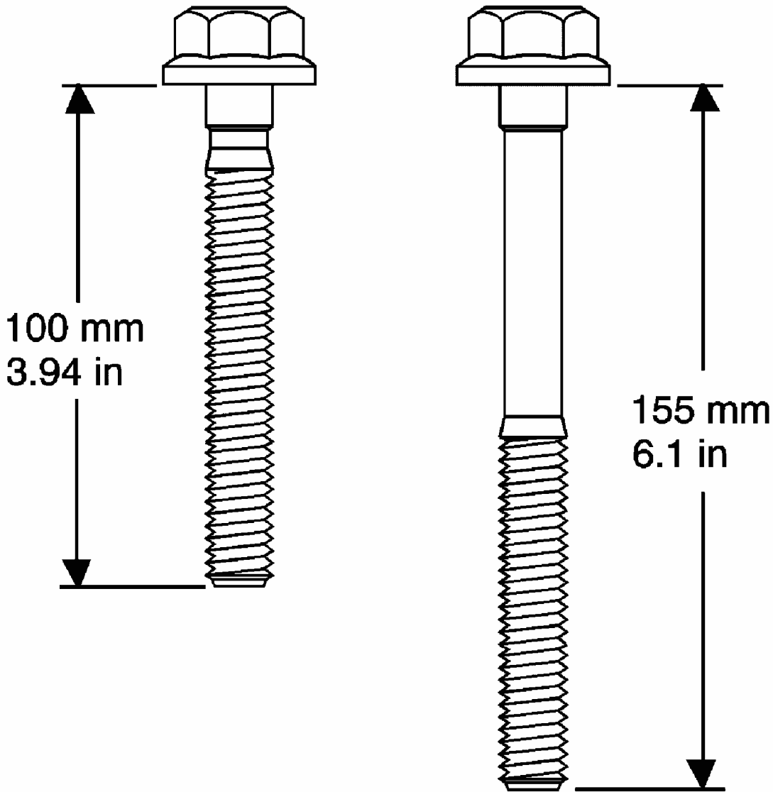
Fig. 166: View Of 100 mm & 155 mm Cylinder Head Bolts Courtesy of GENERAL MOTORS CORP.
