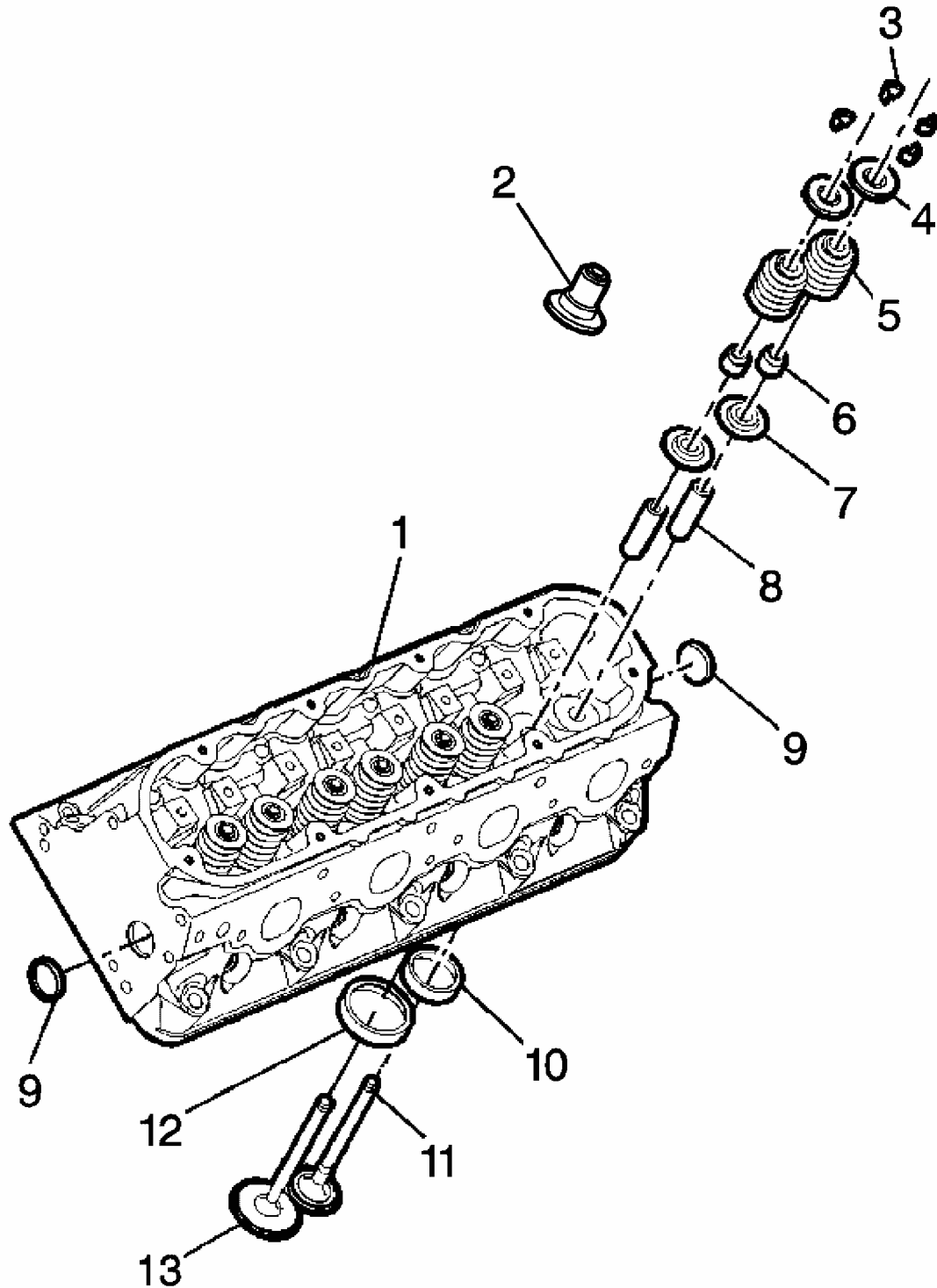
Fig. 144: Valve Stem Keys Courtesy of GENERAL MOTORS CORP.
