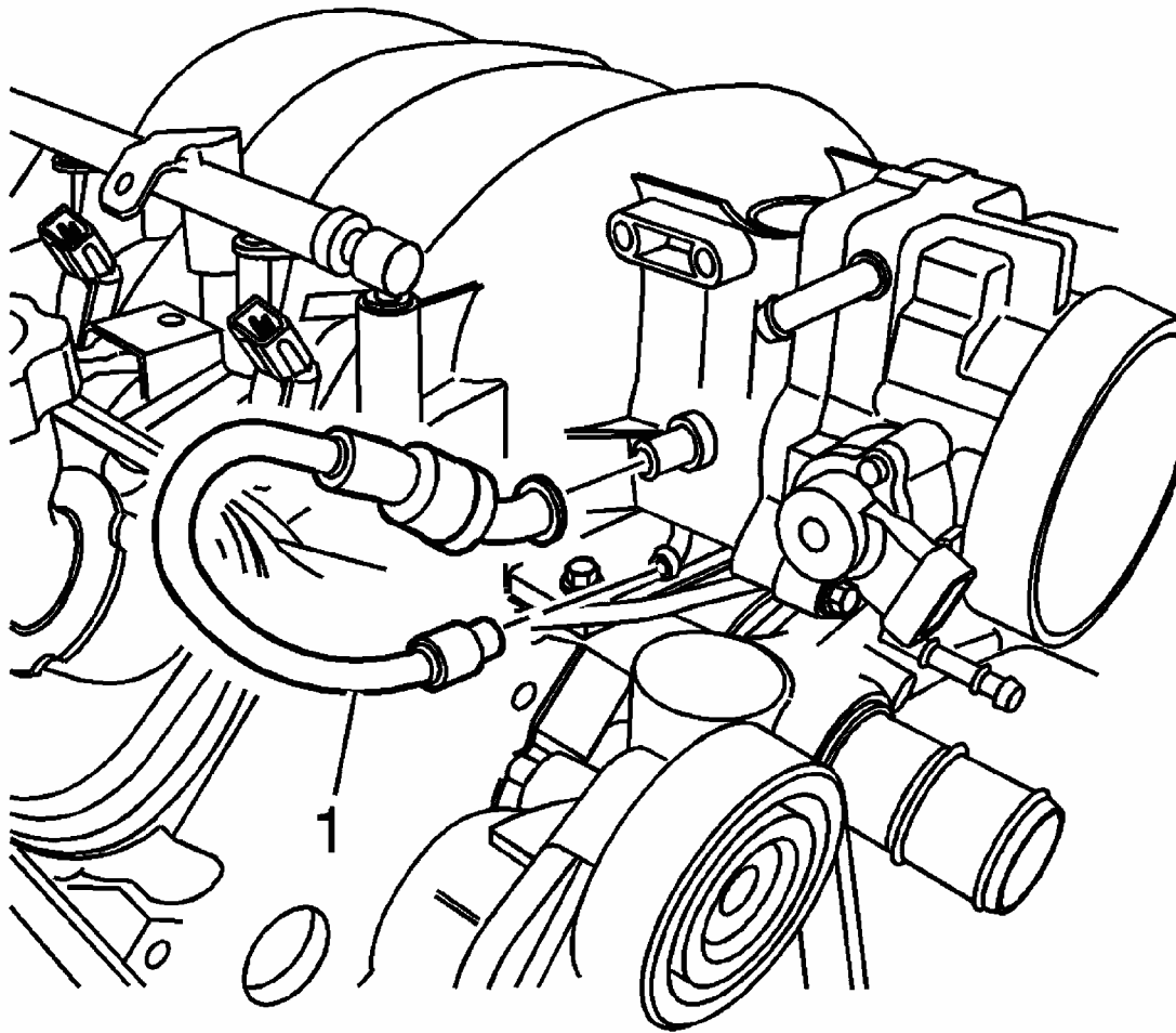
Fig. 33: PCV Valve Hose Courtesy of GENERAL MOTORS CORP.
