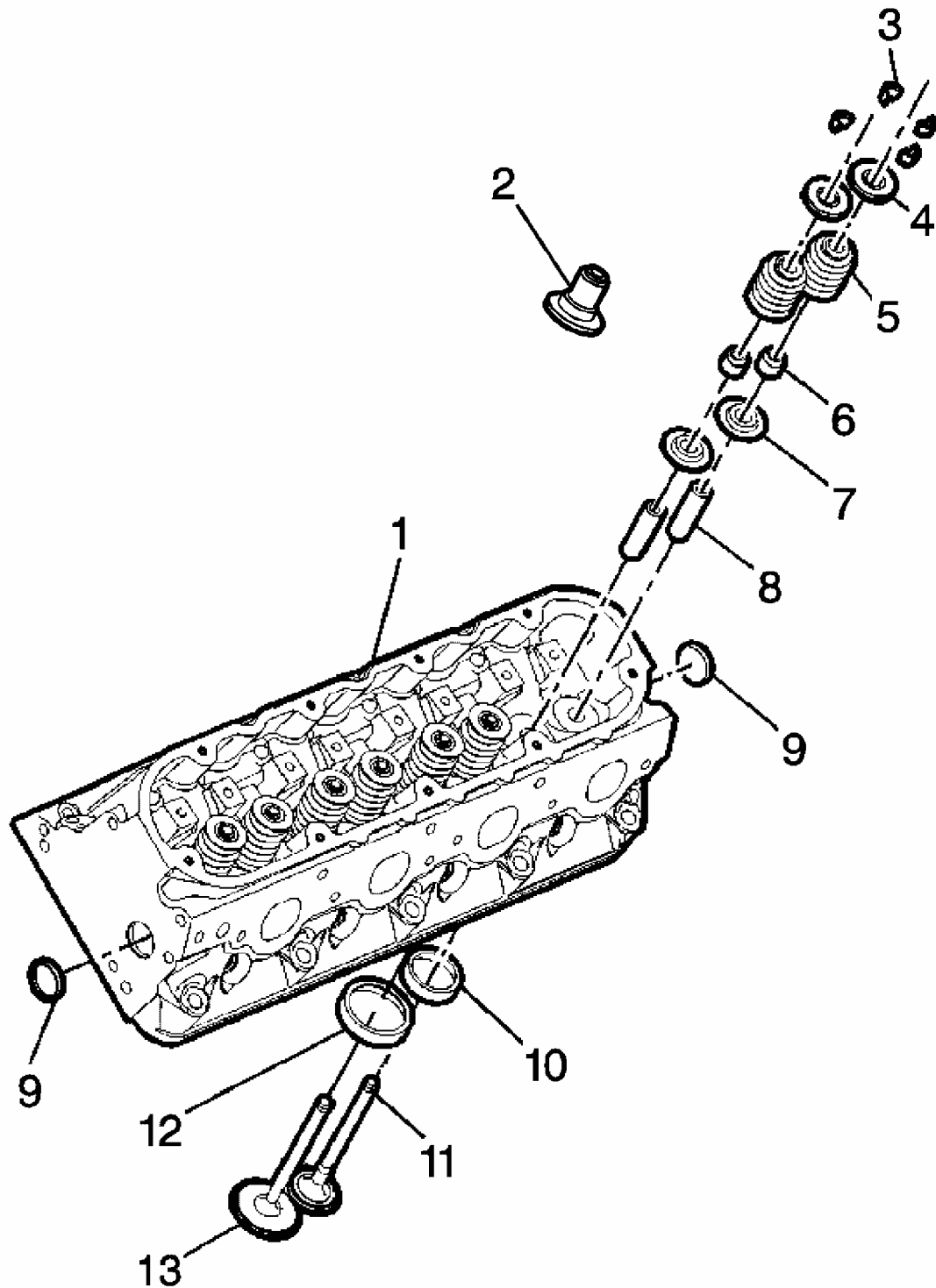
Fig. 140: Valve Stem Keys Courtesy of GENERAL MOTORS CORP.
