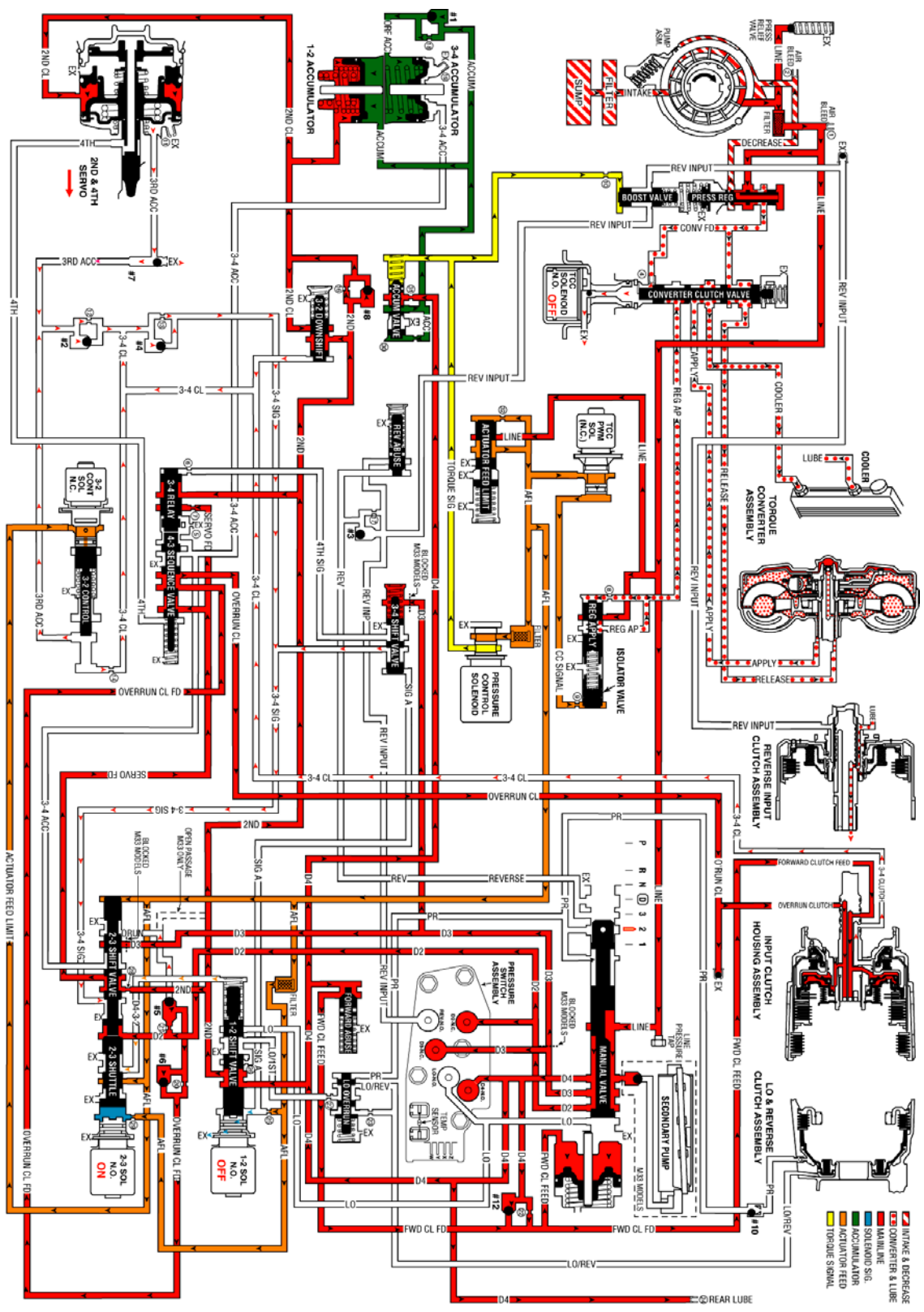
Fig. 11: Manual Second Gear Courtesy of GENERAL MOTORS CORP.
