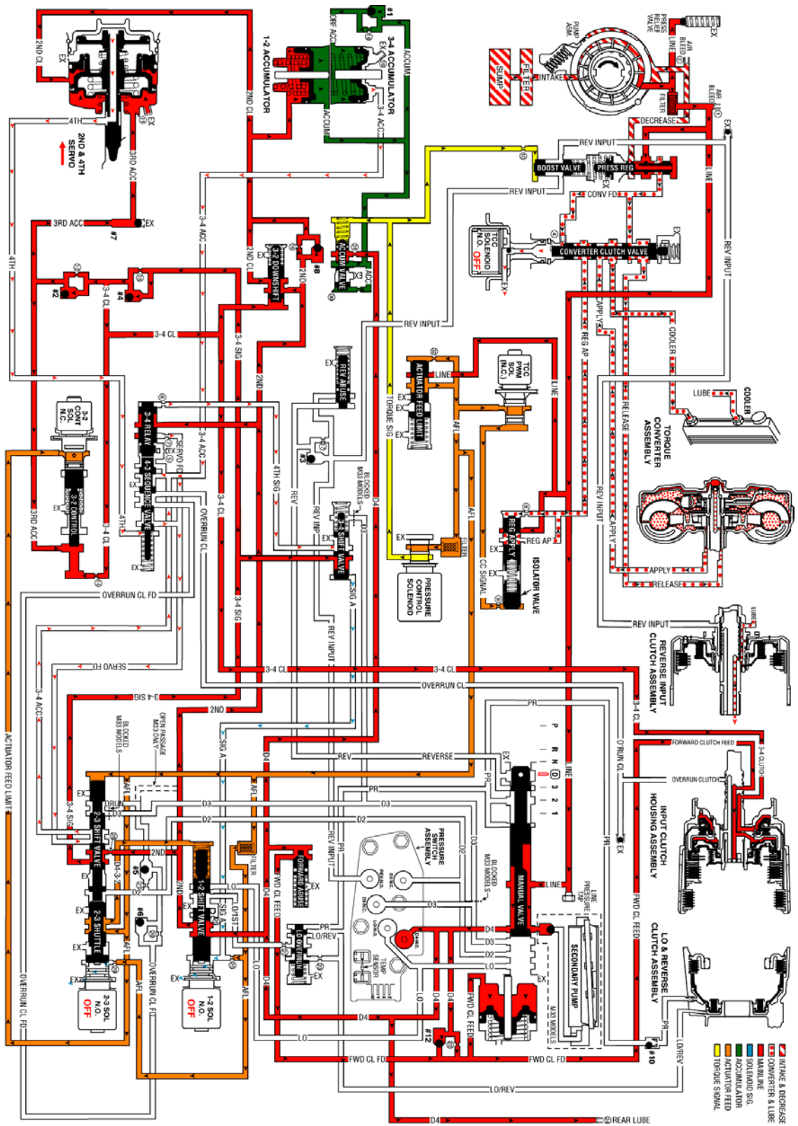
Fig. 8: Overdrive Range, 4-3 Downshift Courtesy of GENERAL MOTORS CORP.
