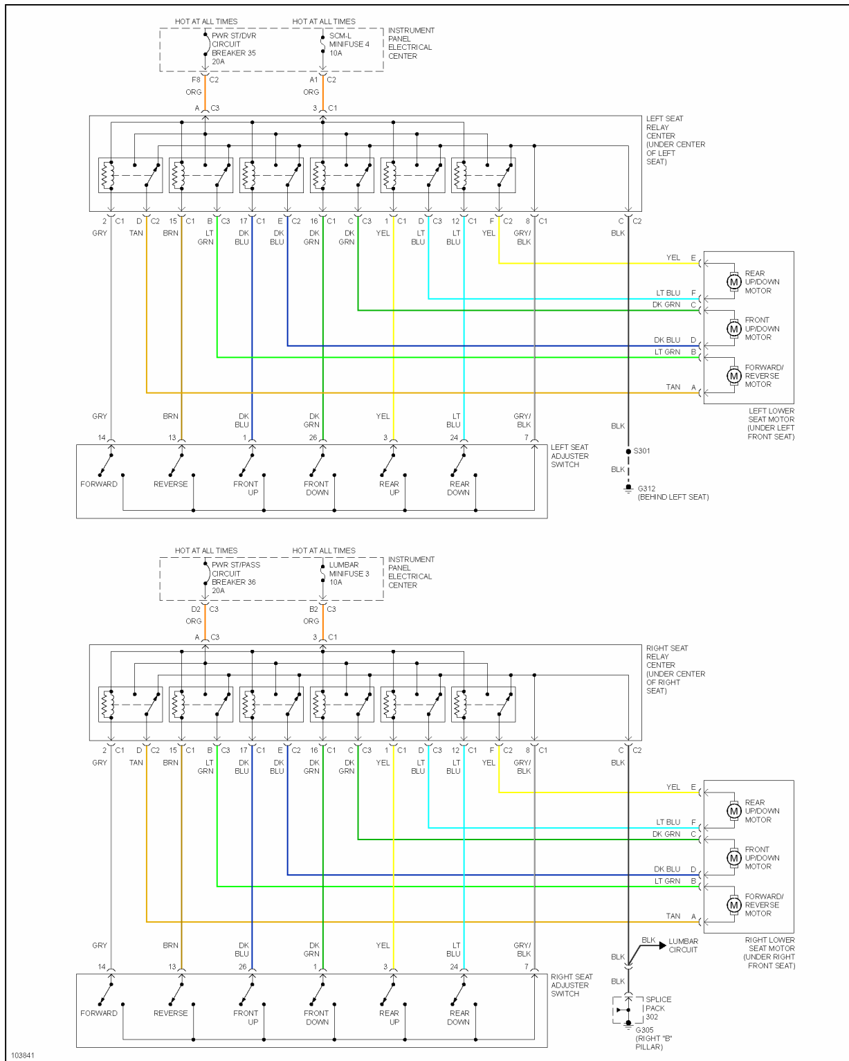
Fig. 7: Power Seats Wiring Diagram
