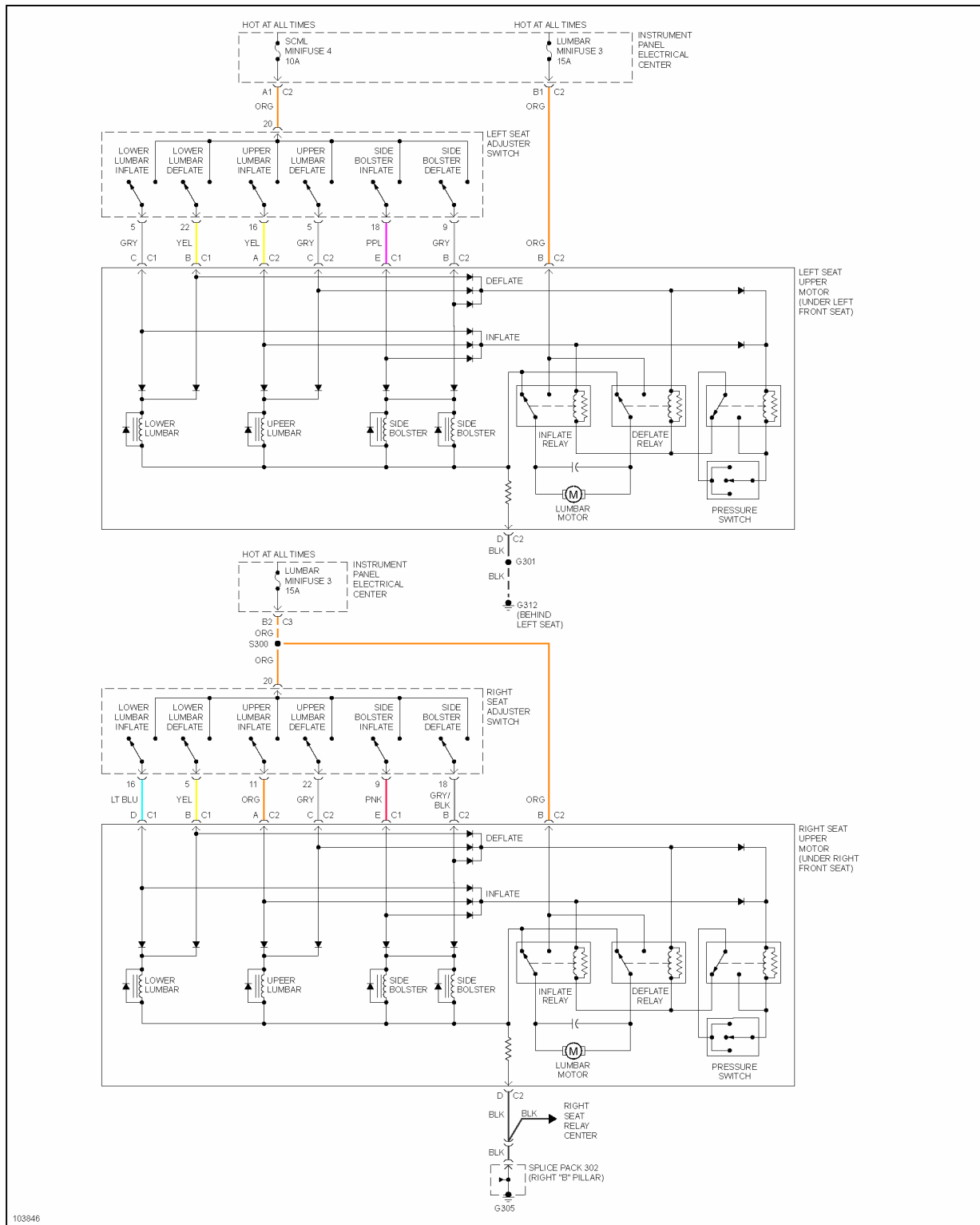
Fig. 8: Power Lumbar Seats Wiring Diagram
