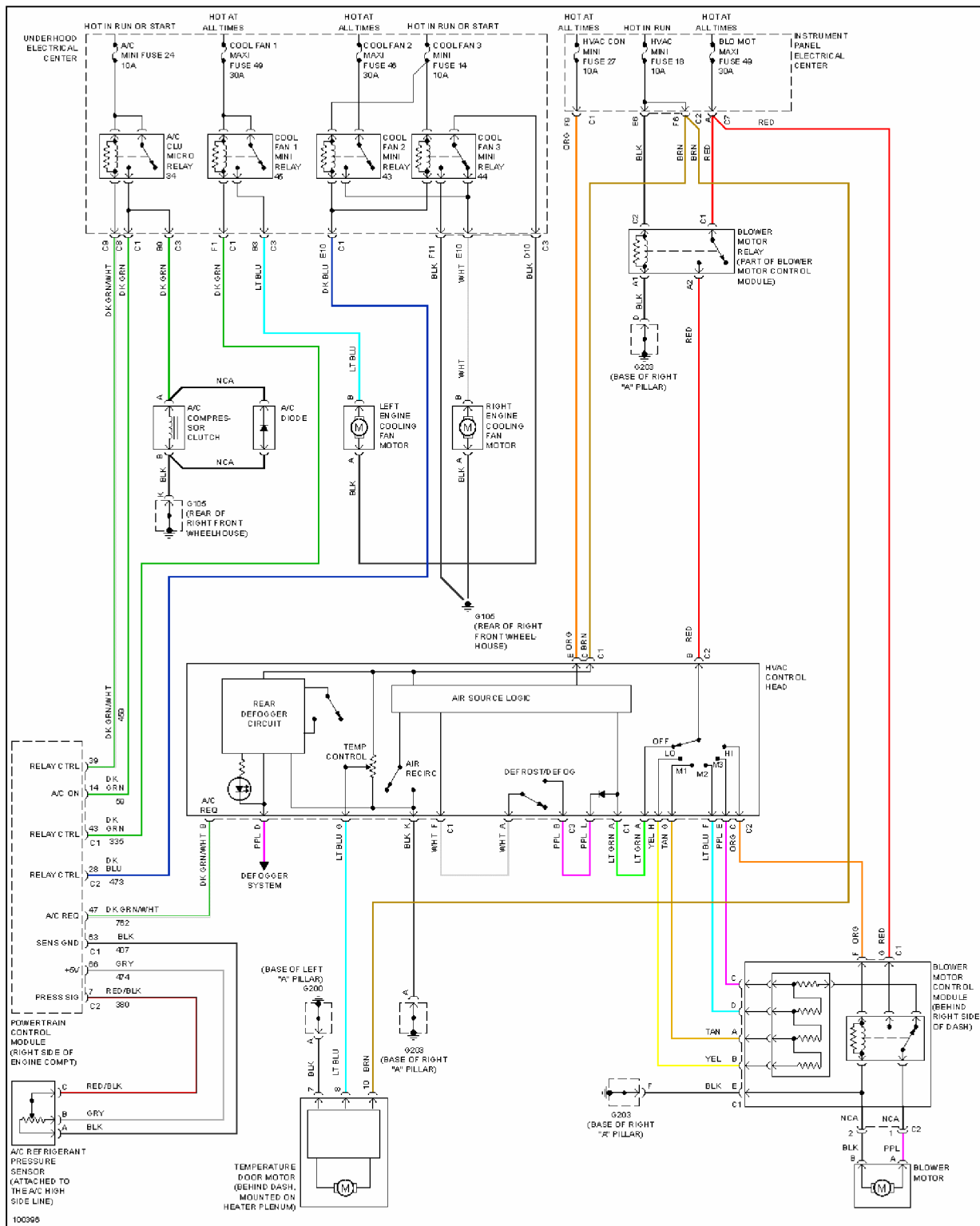
Fig. 2: A/C Circuit, Manual A/C
