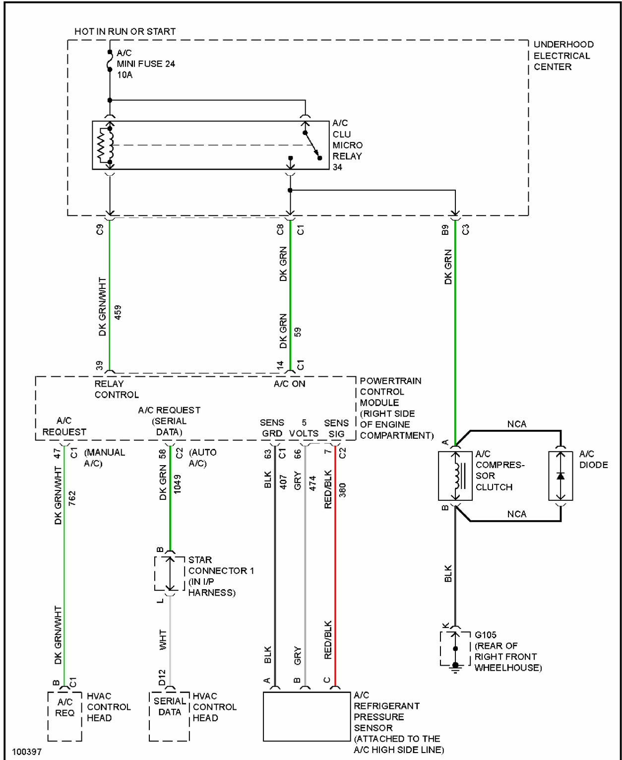
Fig. 3: Compressor Circuit
